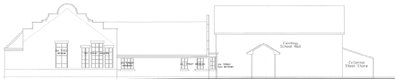
EXISTING EAST ELEVATION.
